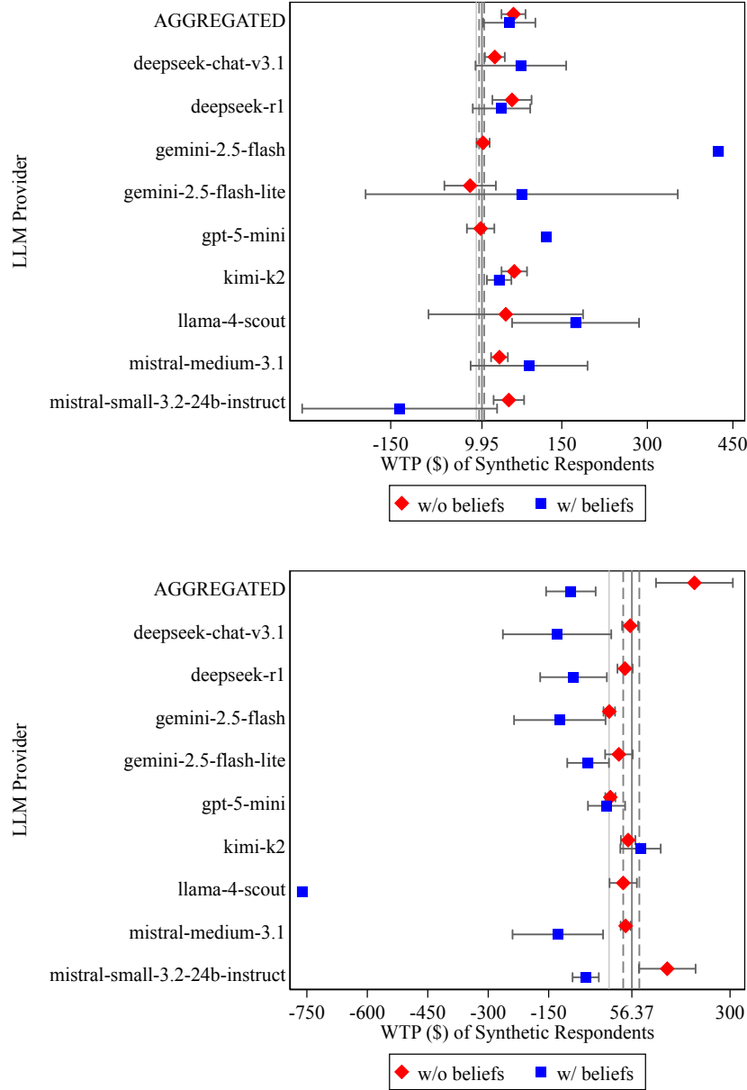
Figure 7: Mean WTP estimates for HWA policy by LLM
